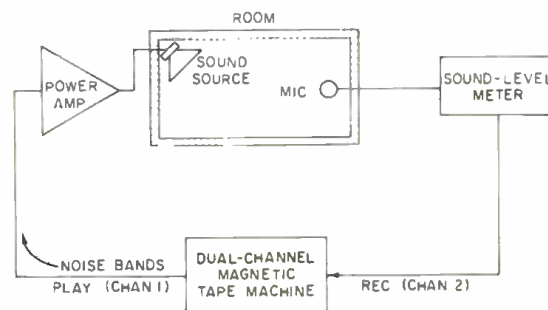
Figure 5. Recording of reverberation characteristics on magnetic tape for later analysis.
