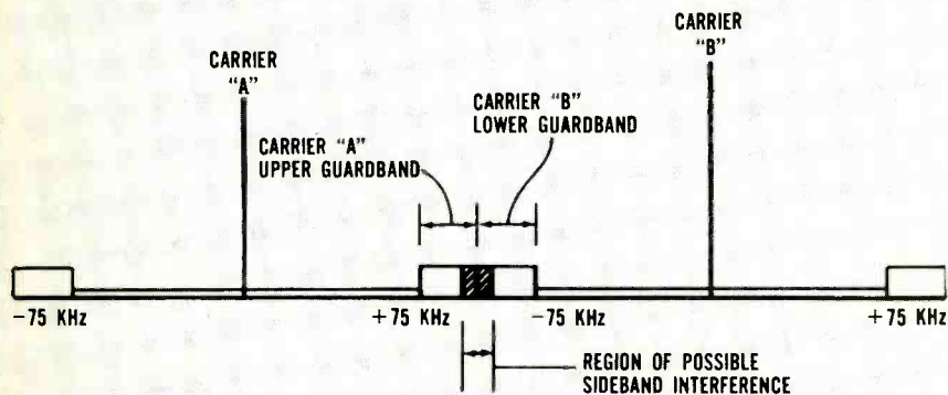
Fig. 2—Under actual conditions described in the text, fully 25 kHz of sideband interaction will take place between the two adjacent channels shown here.
