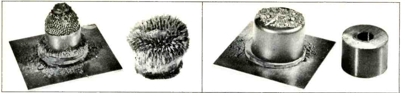
Fig. 10 —Microphones should be protected against environmental hazards. Metallic filings at left, for example, can reach the inner mechanism of a microphone with inadequate protection. In contrast, a properly-protected microphone at right does not allow foreign objects to damage delicate mechanism.
