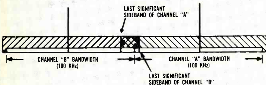
Fig. 2—Under actual conditions described in the text, fully 25 kHz of sideband interaction will take place between the two adjacent channels shown here.
