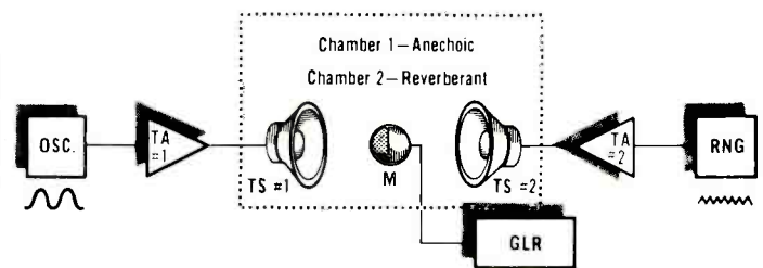
Fig. 9—Four-way test of effective use of a cardioid-pattern microphone tested as an omnidirectional unit.
