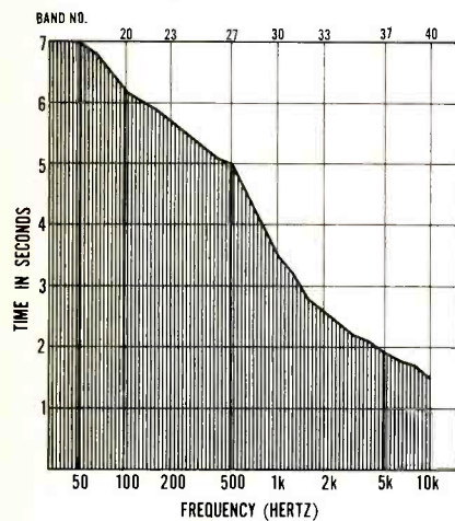
Fig. 8—Reverberation time vs. frequency in a large Catholic church.
