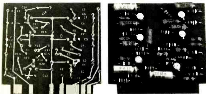
Fig. 8—Front and back views of the small etched circuits used to construct the electronic crossover unit.
