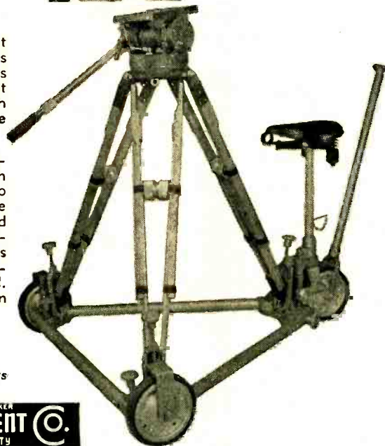
Below: 3 wheel portable dolly with balanced TV Tripod mounted.
