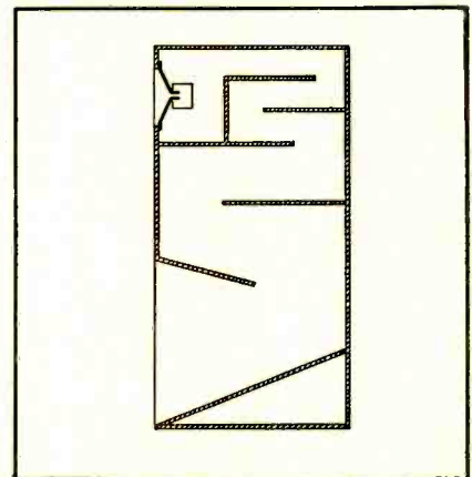
Fig. 3. Conventional acoustic labyrinth which utilizes a folded horn for the back wave.
