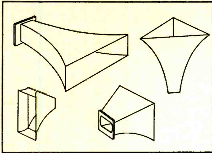
Fig. 2. Possible configurations of exponential flares.
