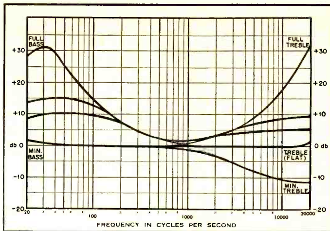
Fig. 4. Response curves of the tone control section.
