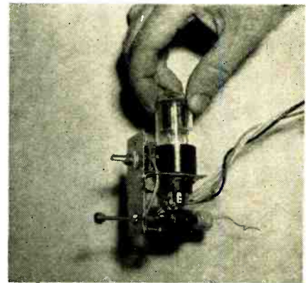
Fig. 2. View of scratch filter chassis ready for installation in existing amplifier.
