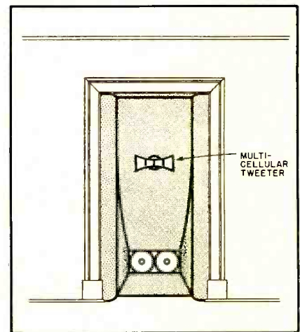
Fig. 6. Full-sized straight horn suitable for closet or doorway installation.
