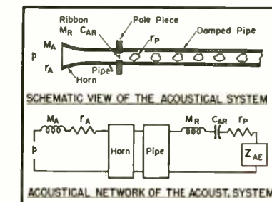
Fig. 3. Acoustical system and network of a pressure-type ribbon microphone with a horn coupled to a cylindrical pipe as the sound pickup means.
