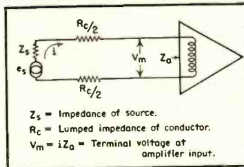
Fig. 1. Example of a metallic circuit voltage.
