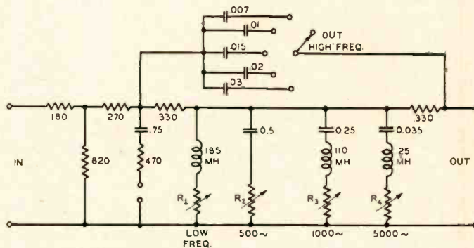
Fig. 3. Circuit of crossover filter.
