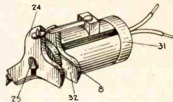
Fig. 4. Polyphase reproducer arranged for mounting of three styli. As shown, upper stylus is for lateral records, one at lower left is for vertical transcriptions.
