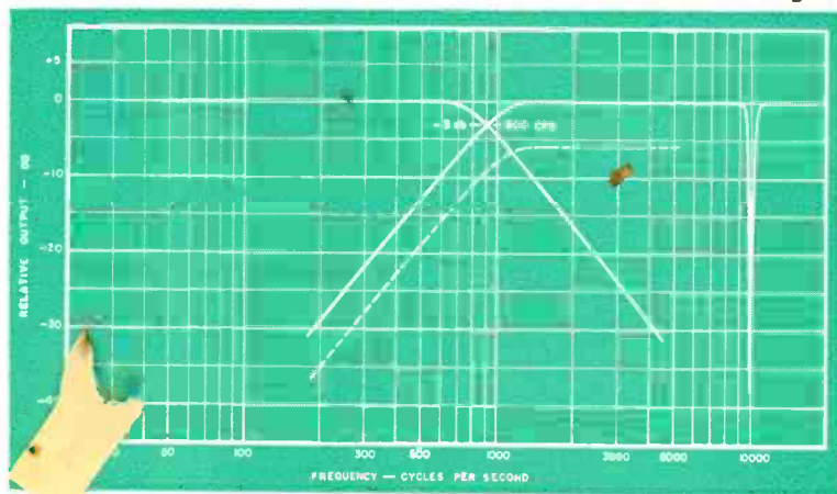
Fig. 6. Curves of typical response from dividing network, and attenuation to be expected from 10-kc suppressor. Dotted curve shows range of adjustment furnished by 1 db/step attenuator.
