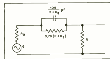
Fig. 7. Interstage equalizer for flat response from G. E. or similar magnetic pickups. R_0 represents the internal resistance of the driving amplifier.
