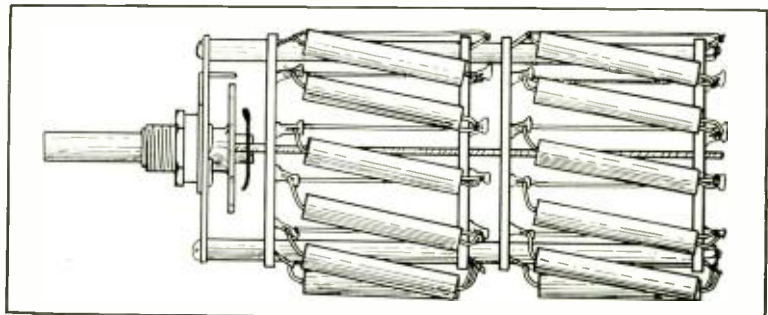
Fig. 2. Method of arranging switch sections to support the resistors for the 1 db/step attenuator in the h-f speaker circuit.
