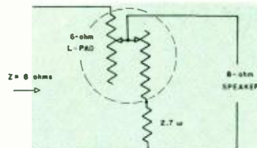
Fig. 4. Alternate arrangement showing the use of a 6-ohm L-pad in an 8-ohm circuit to provide a maximum loss of 12 db.
