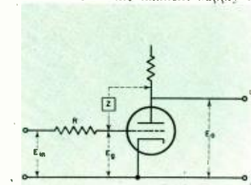
Fig. 2. Detail of feedback stage. Z represents the network R_5 , C_3 and C_4 of Fig. 3. R is approximately equal to R_4 .
