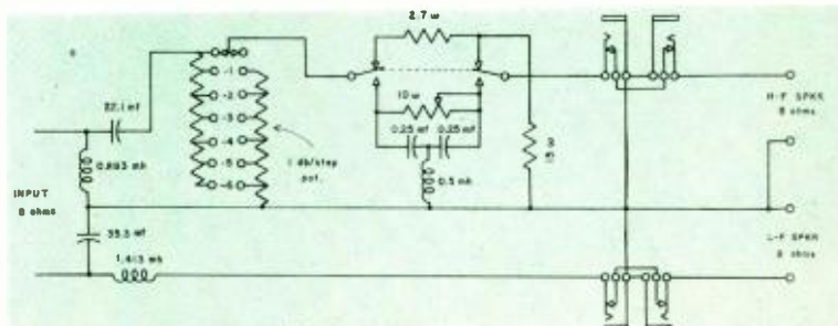
Fig. 6. Complete circuit of dividing network, h-f attenuator, 10-kc suppressor, and jacks to permit access to the various circuits.
