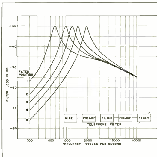
Fig. 6 (left). Typical telephone filter characteristics. Fig. 7 (right.) Echo chamber line-up.
