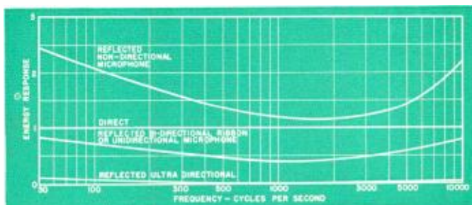
Fig. 2. Energy response curves for direct and reflected sounds in a typical studio
