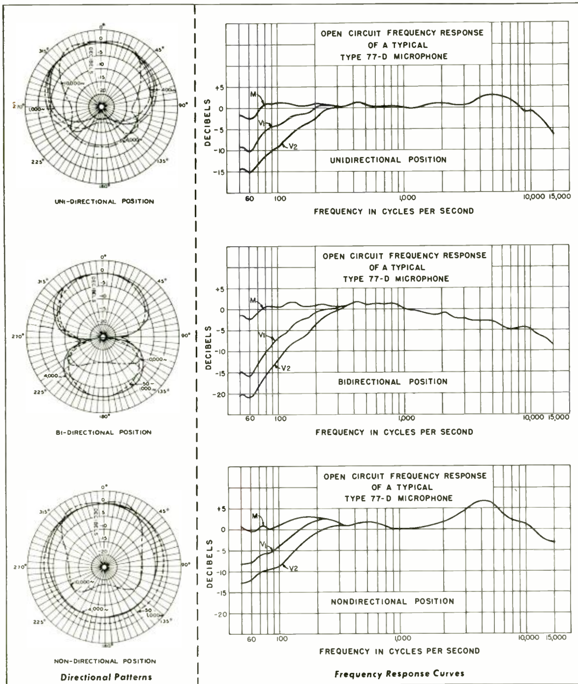
Fig. 5. Directional patterns and frequency response curves for the RCA Type 77-D microphone.
