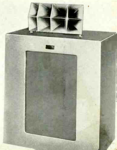
Fig. 8. Typical mounting of two-way speaker system, commercially available. Courtesy Stephens Manufacturing Co. Inc.
