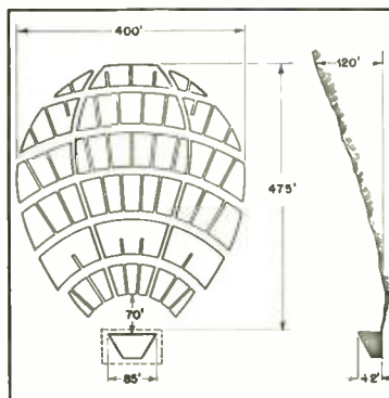
Fig. 1. Layout of the Hollywood Bowl. The stage for the orchestra is at the lower end of the drawing.
