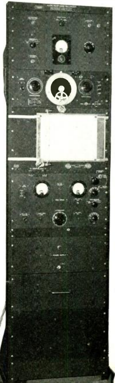
Fig. 3. Automatic audio response recorder.
