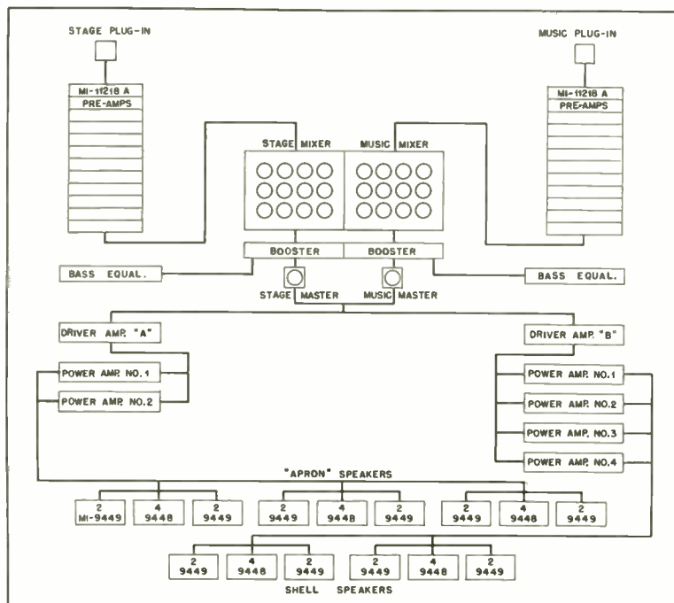
Fig. 2. Block diagram showing arrangement of sound equipment.
