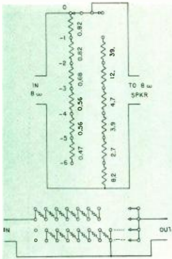
Fig. 3. Circuit arrangement for h-f attenuator, showing resistor values for an 8-ohm circuit.
