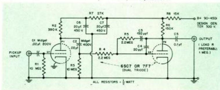
Fig. 3. Complete schematic of the magnetic pickup preamplifier, using negative feedback over the second stage to accomplish equalization.
