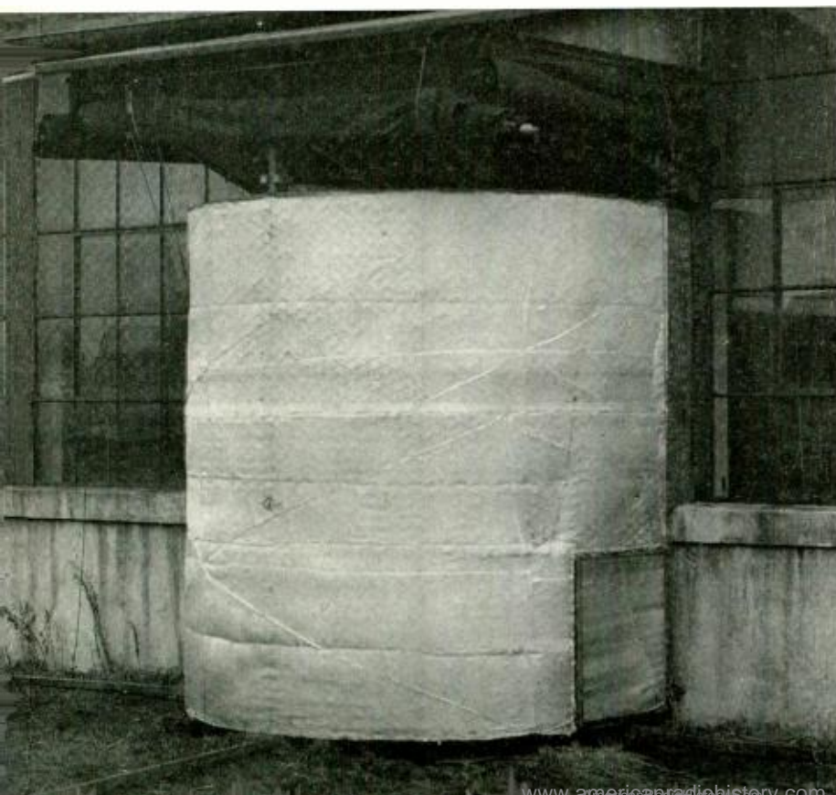
Fig. 1. Outdoor measuring set-up. Two layers of parachute cloth one inch apart serve as a windscreen transparent to sound. The speaker is mounted on a baffle flush with the wall and the microphone supported on an adjustable boom in front of the speaker.
