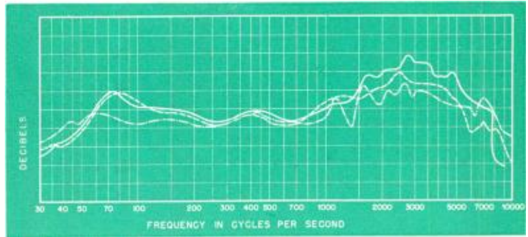
Fig. 6. On-axis response of typical 12" speakers. (Below).
