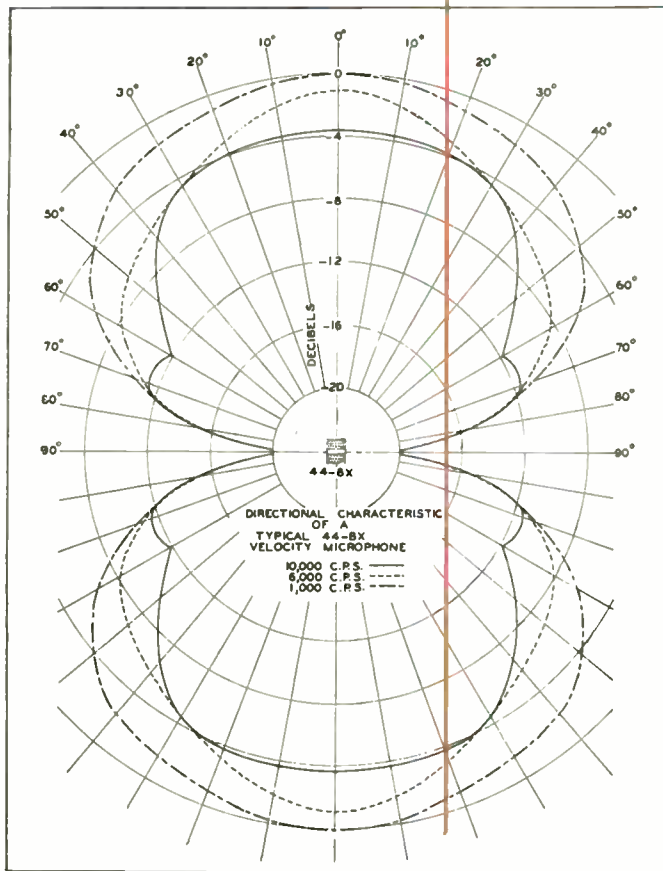
Fig. 4. Directional characteristics of the RCA Type 44-BX microphone.
