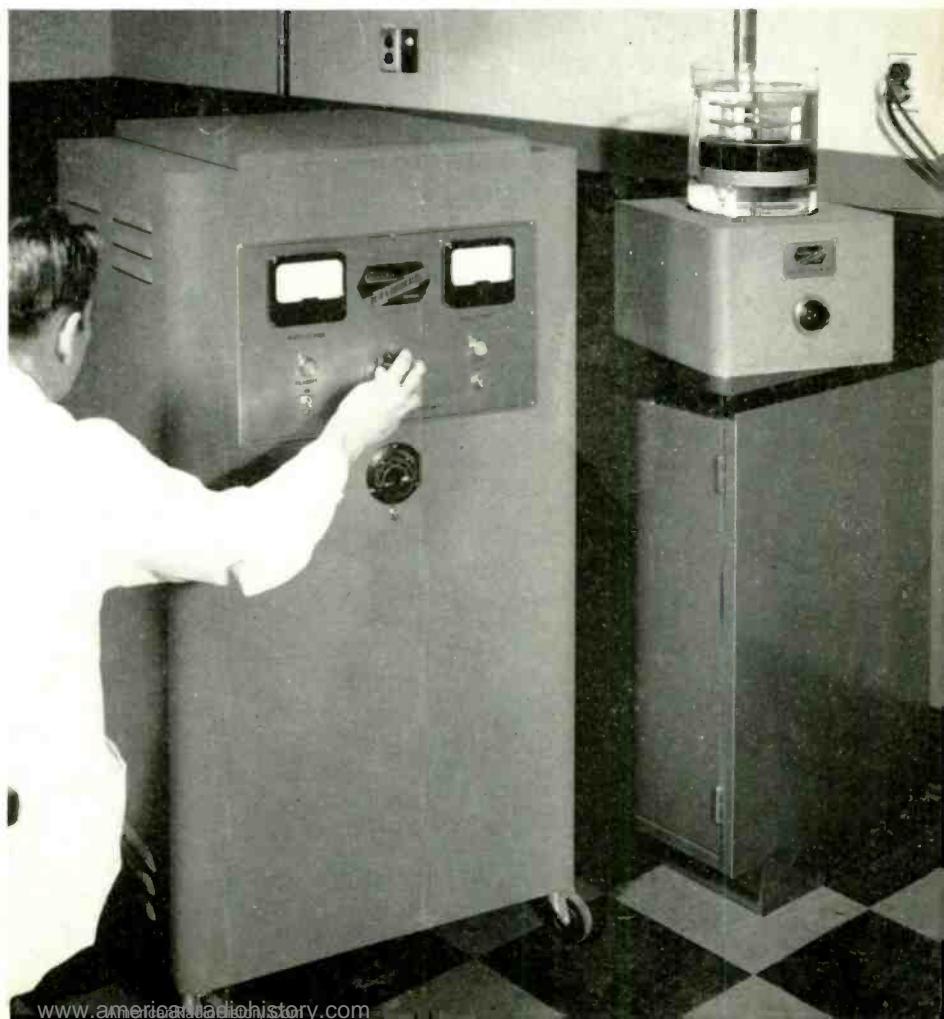
Crystal ultrasonic generator providing 600 watts into final stage. Four frequencies, from 400 kc to 1200 kc, are provided. (Courtesy Eimer and Amend)
