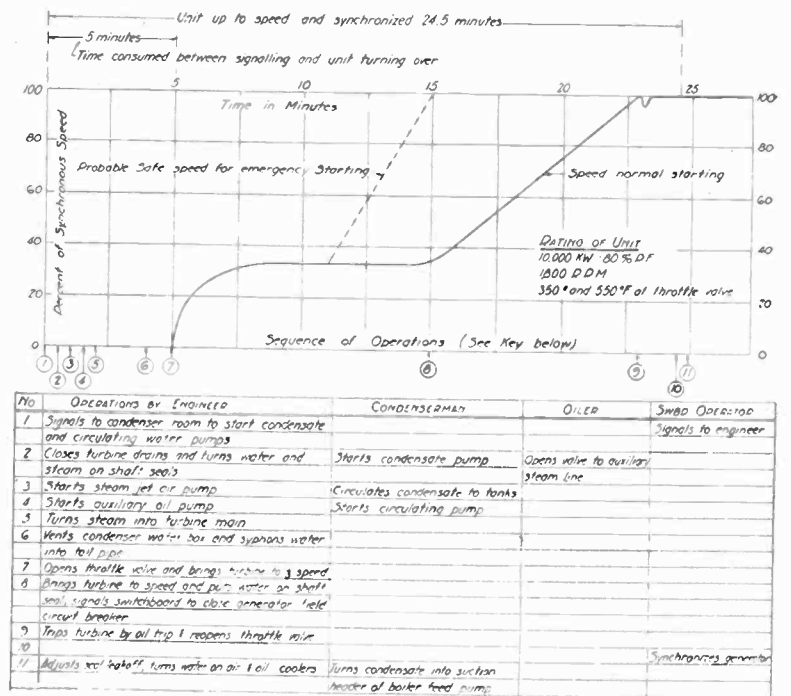
FIG. 6—ANALYSIS OF TIME CONSUMED IN STARTING A 10,000-KW. STEAM UNIT
