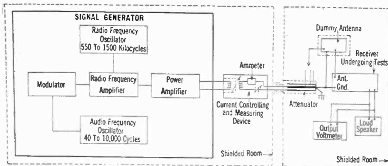
FIG. 1—SCHEMATIC LAYOUT OF RECEIVER TEST APPARATUS
