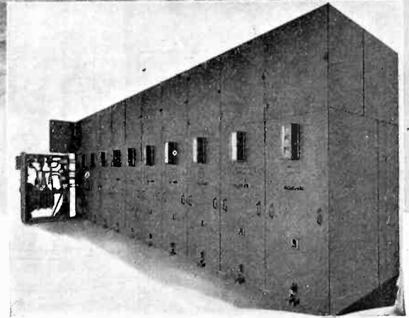
Safety Enclosed Switchboard, Removable Truck Type
