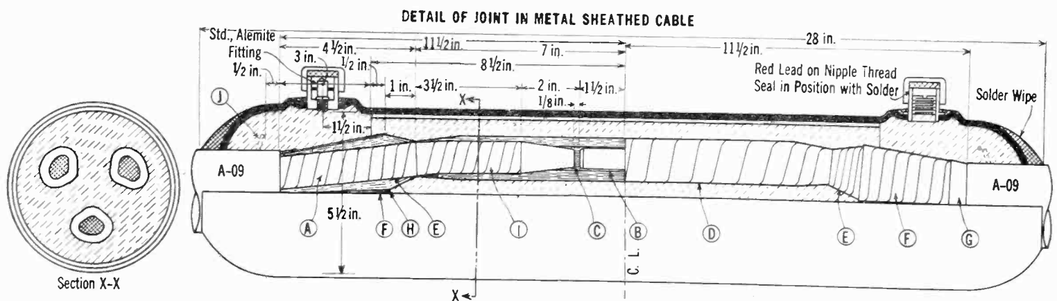
FIG. 4—SPECIFICATIONS FOR 3-CONDUCTOR, 27,000-VOLT, 09 CABLE JOINT 27-3
