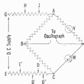
FIG. 5—RESISTOR OPERATION
