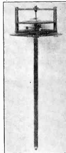
FIG. 2—COMPASS FLUXMETER
