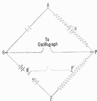
FIG. 3—BATTERY OPERATION
