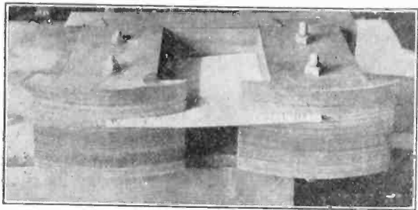
FIG. 3—EXPERIMENTAL SET-UP OF ALTERNATOR FIELD POLES
