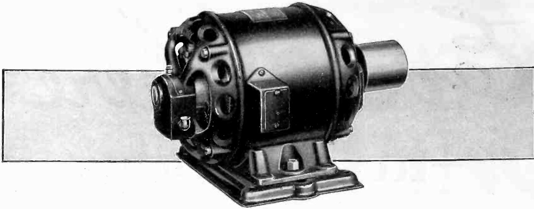
1/8 horse-power Century Type RS Repulsion-start Induction Single-phase Motor
