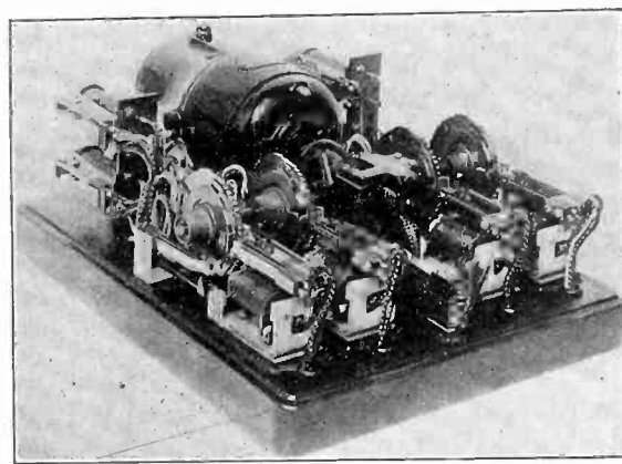
FIG. 2—SUBSTATION MOTOR SENDING KEY
