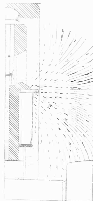
FIG. 5—MAGNETIC LEAKAGE FLUX AT ONE END OF A POLE OF A 6-POLE, 435-KV-A., 1200 REV. PER MIN., 4000-VOLT ALTERNATOR
