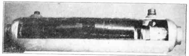
FIG. 2—CUT-AWAY OF JOINT IN BELTED CABLE
