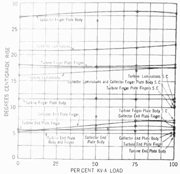
FIG. 11—TEMPERATURE RISES ABOVE INGOING AIR OF FINGER PLATES, END PLATES AND LAMINATIONS, NON-MAGNETIC END PLATES (Generator No. 3)
