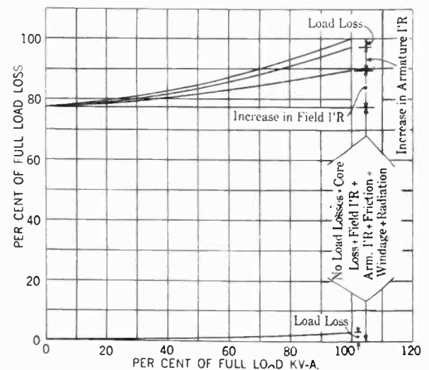
FIG. 5—SHOWING RATIO OF LOSS TO LOAD (Generator No. 3, 3125-kv-a., 2300-volt, three-phase, 60-cycle, 3600-rev. per min.)
