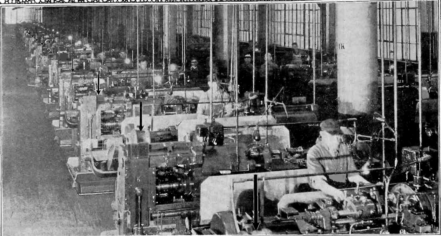
A partial view of one hundred and six "automatics" operated by as many New Departure Ball Bearing equipped General Electric motors. These have been in operation from 8 to 10 hours per day for 20 months without adding to the original lubricant placed in the bearing housings by the motor manufacturer at the time of assembly.
