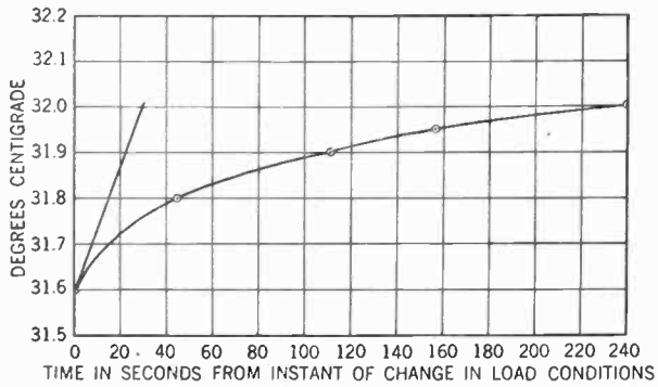
FIG. 14—TEMPERATURE RISE OF IRON VS. TIME
