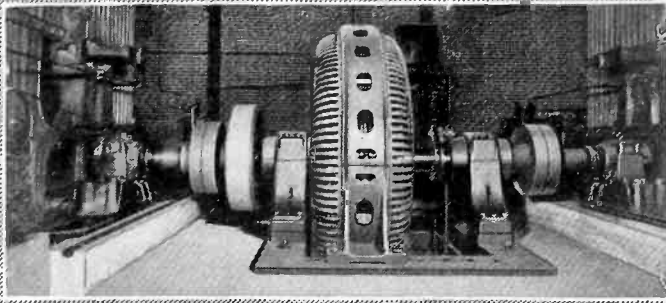
PULP GRINDER DRIVE
