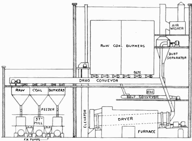
FIG. 4—LONGITUDINAL SECTION THROUGH COAL PREPARATION PLANT
