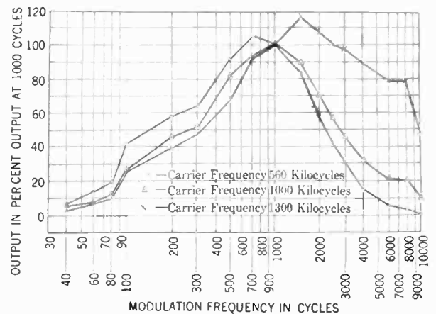
FIG. 6—CURVES SHOWING THE RELATION BETWEEN VOLTAGE ACROSS THE LOUD SPEAKER AND MODULATION FREQUENCY WHEN THE FIELD STRENGTH AND DEGREE OF MODULATION ARE HELD CONSTANT
