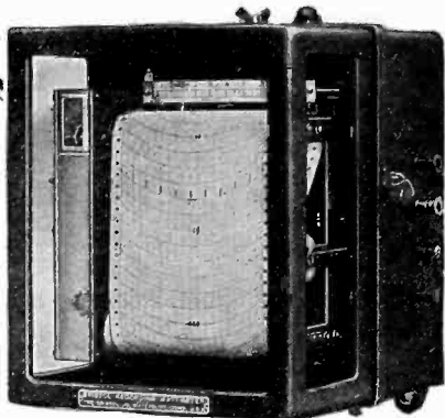
Bristol's Recording Wattmeter
