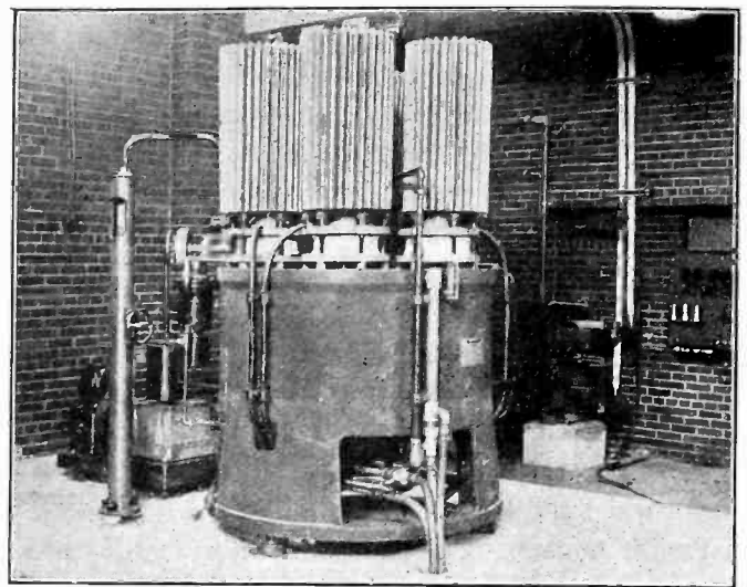
FIG. 5—SHOWING RECENT INSTALLATION OF A 1000-AMPERE, 600-VOLT, D-C. RECTIFIER
