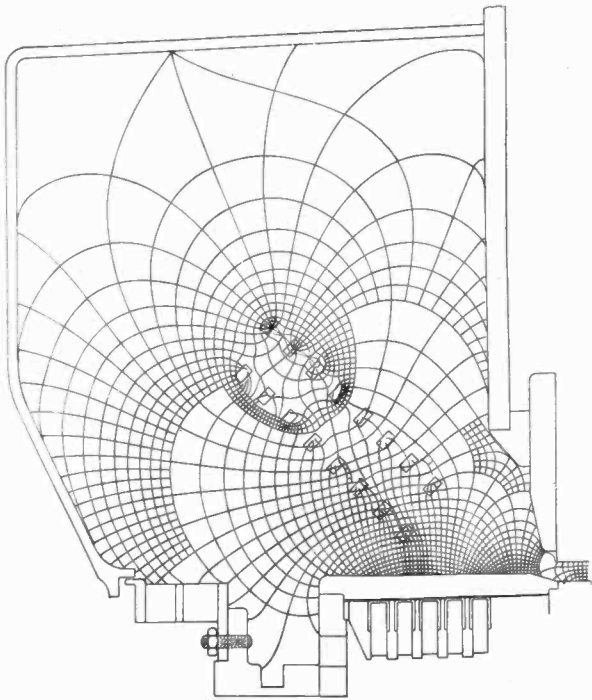
FIG. 20—TURBO GENERATOR END BELL LEAKAGE FLUX. Three-phase diamond coil armature winding section through radial plane of maximum flux densities for full load voltage and zero per cent power factor with armature current of 0.866 maximum value in two phases and zero in the third.
