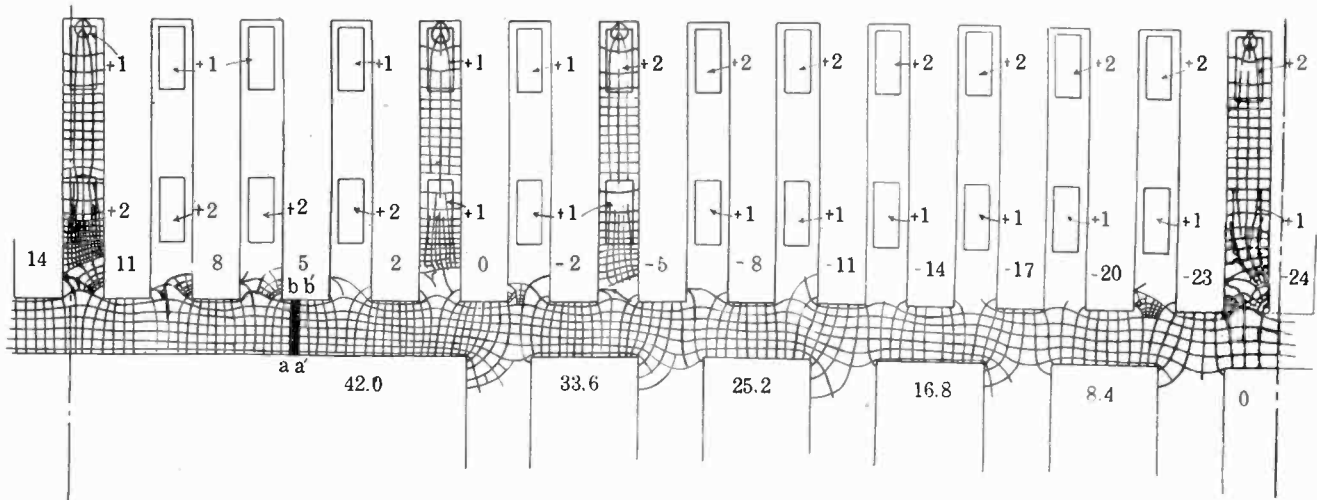
FIG. 19—TOTAL ARMATURE AMPERE-TURNS PER POLE = 13,200 AND ARE TAKEN AS PROPORTIONAL TO 25 IN THESE CALCULATIONS Total field ampere-turns per pole = 22,277 and are taken as proportional to 42 in these calculations. Per inch perpendicular to the sheet the flux per tube a - a' to b - b' = 3.19 \times 13,260 \times \frac{5}{25} = 8460 lines
