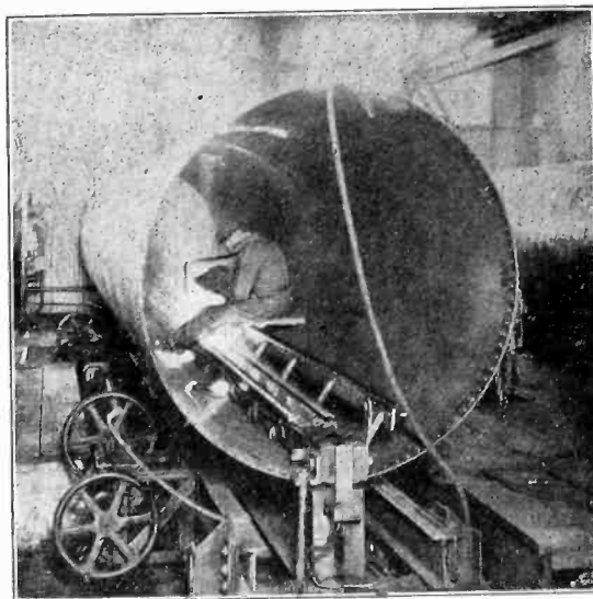
THIRTY-FOOT SECTION OF PIPE IN TESTING MACHINE
