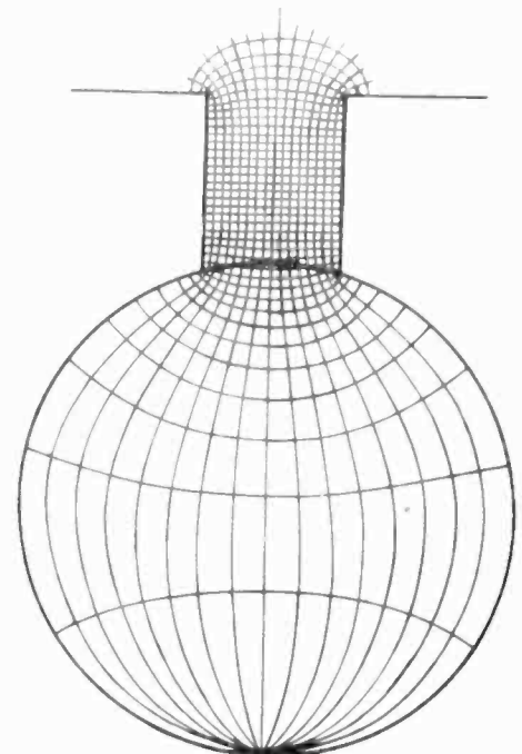
FIG. 13—FLUX DISTRIBUTION ACROSS A ROUND SLOT WHEN THE CONDUCTOR IS IN CONTACT WITH THE IRON
