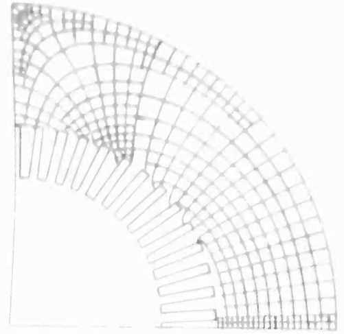
FIG. 11—FLUX DISTRIBUTION IN THE CORE OF A TWO-POLE TURBINE GENERATOR ON THE ASSUMPTION OF UNIFORM PERMEABILITY
