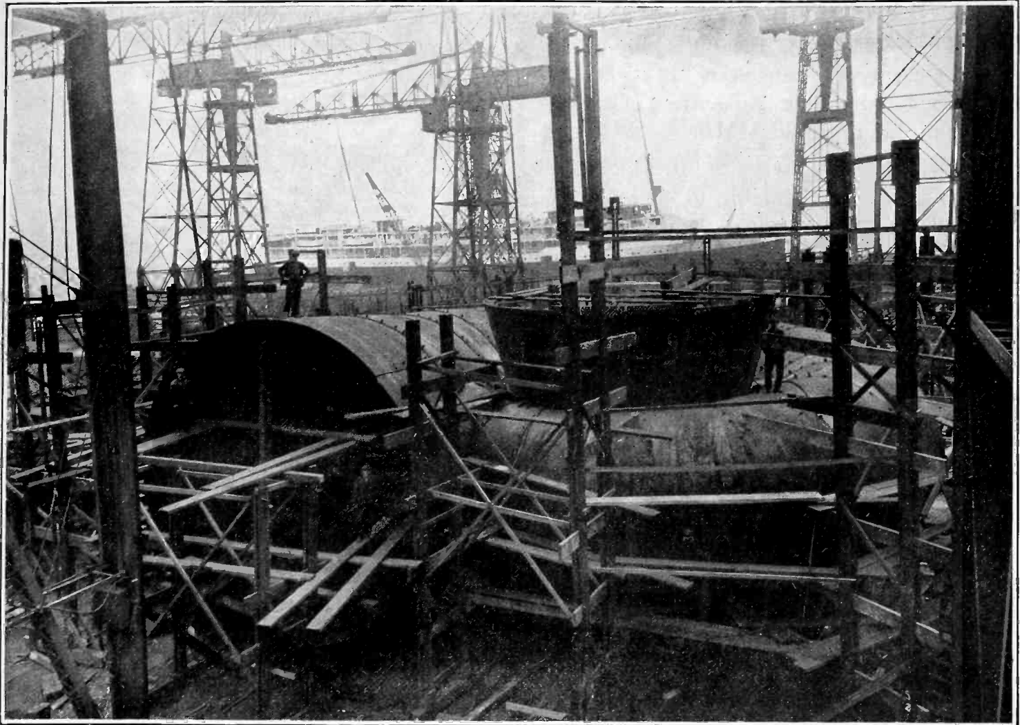
PLATE STEEL VOLUTE CASING FOR ONE OF THE 54,000 HORSEPOWER TURBINES TO BE INSTALLED IN THE SUSQUEHANNA POWER COMPANY'S CONOWINGO DEVELOPMENT HEAD 89 FT. SPEED 81.8 R.P.M.
