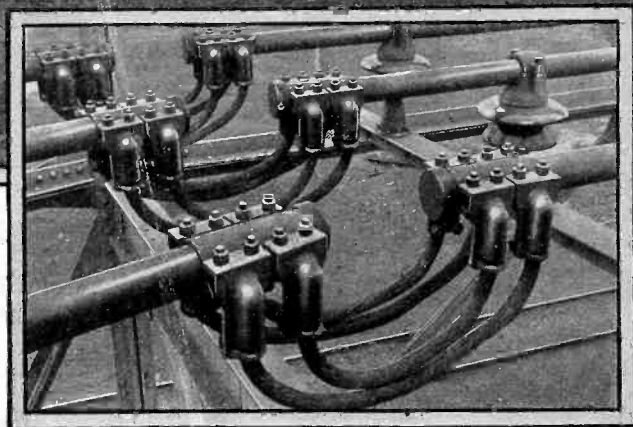
Detail of angle expansion joint
