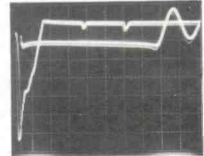
Figure 7(c). As above, but with 100 \mu s/div to show arc duration.
