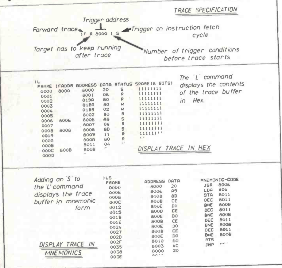
Figure 9. Trace analysis with Microtek's MICE II.
