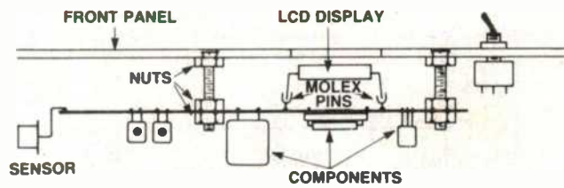
Figure 3. Mounting the pc board.
