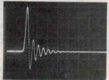
Measured impulse response of Sony D50 compact player.
