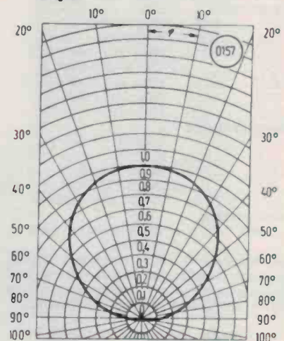
Directional characteristic Short-circuit current versus half angle
