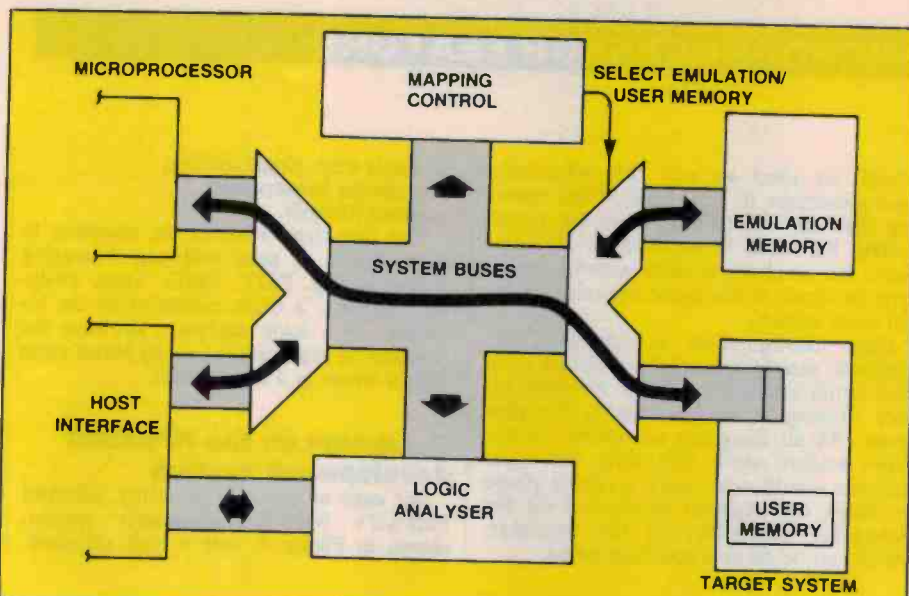
Figure 2. Simplified emulator architecture.
