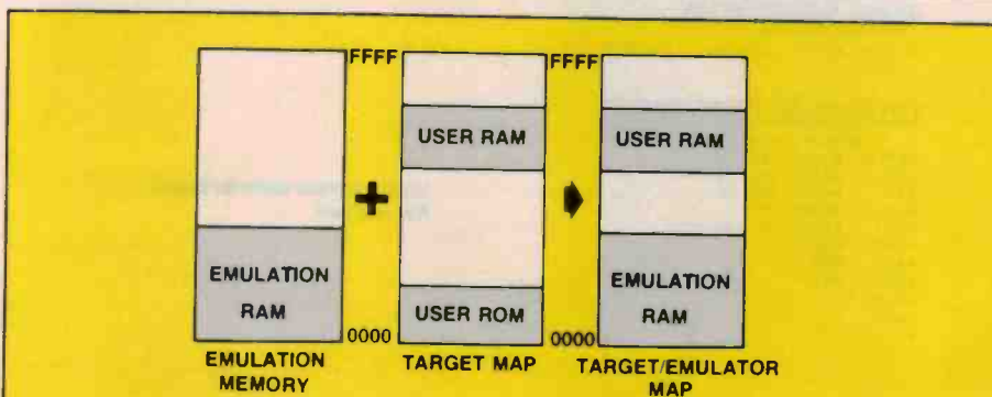
Figure 3. Mapping — constructing memory map for emulation. In this example, 'user ROM' overwritten by emulation RAM, allowing software to be loaded and tested by host system.
