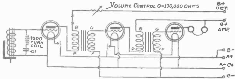
W.W. (Croydon) and F.H. (Sydney) ask for a simple gramophone amplifier. This should suit their requirements admirably. The transformers should have a ratio of 3 1/2 to 1. The 1500-turn coil and .01 condensers constitute an input filter.
