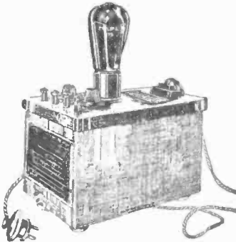
PHILIPS STANDARD 1 "B" ELIMINATOR, 372.
