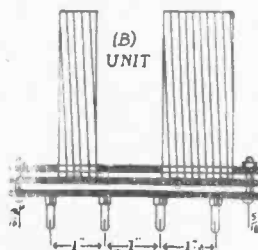
FIG. 4. (b) The complete coil unit to fit the mounting. (c) The aerial coupling coil on its swivel dome.
