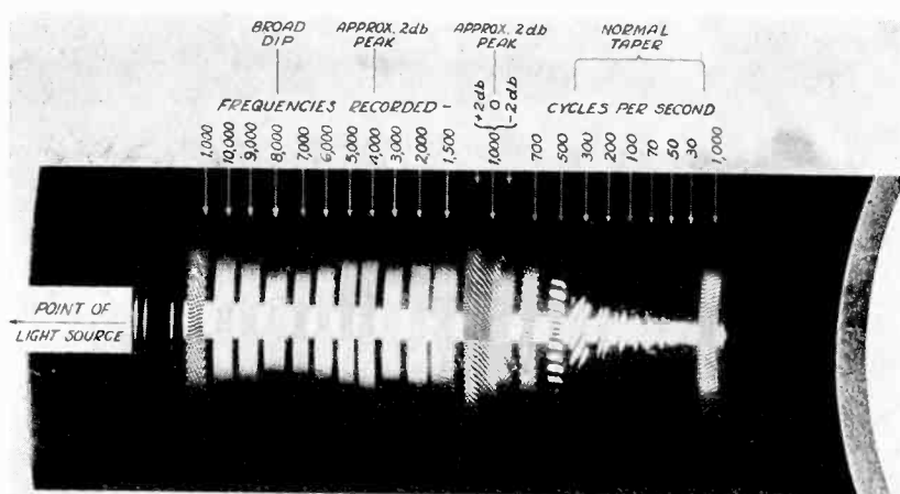
OPTICAL PATTERN OF TYPICAL TONE RECORD
