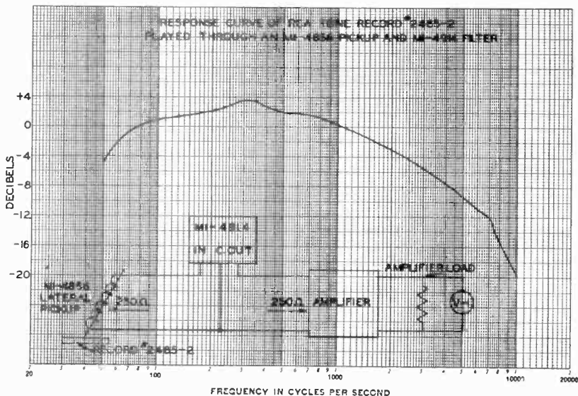
(Below) Performance curves on the MI-4914.
