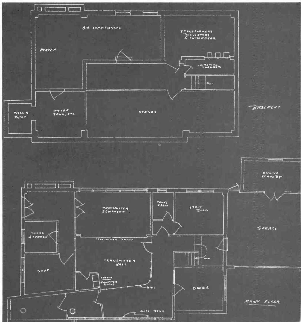
Floor plan of CBM
